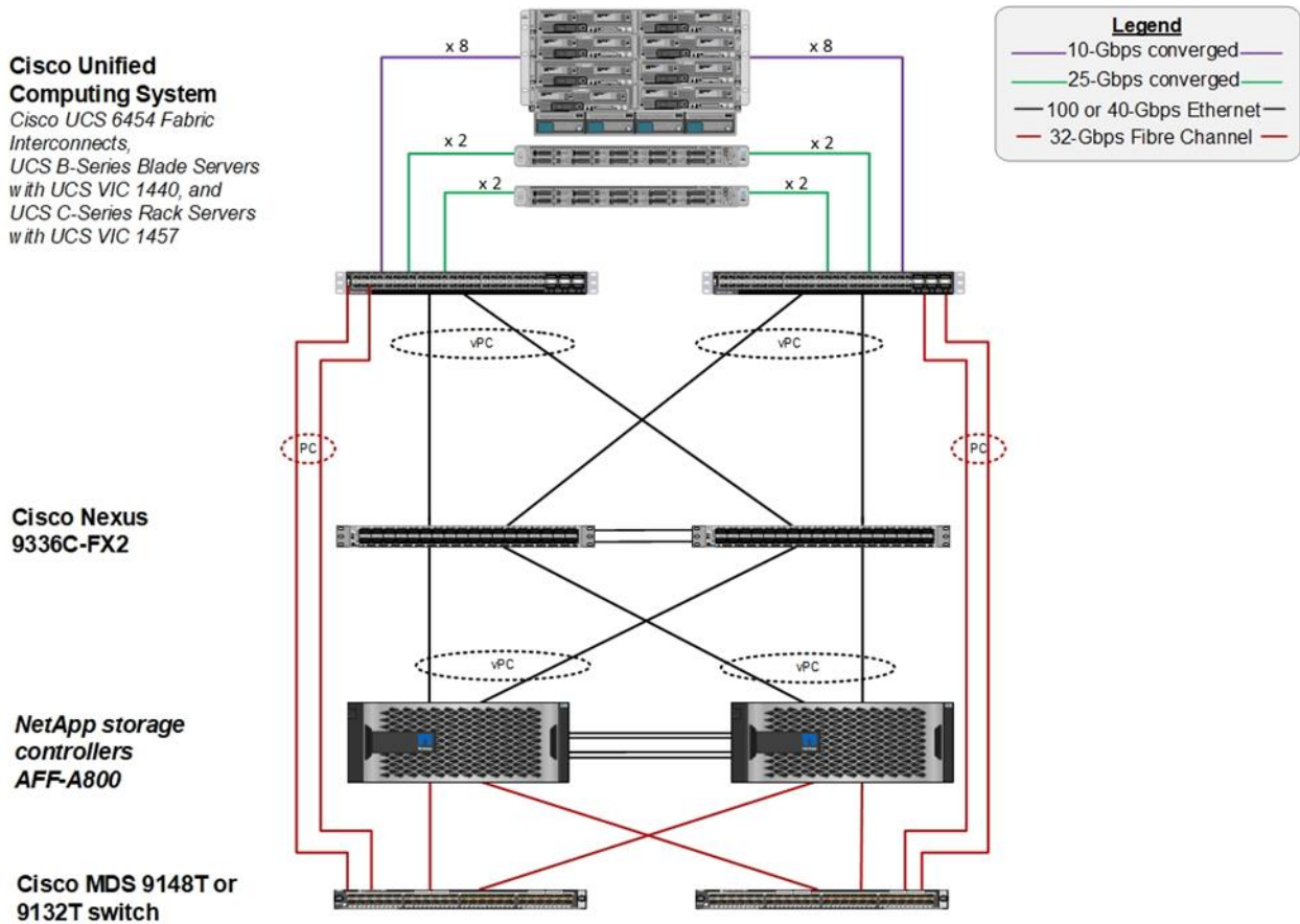
Figure 1) FlexPod architecture.
